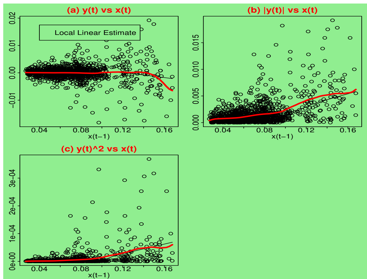
Figure 2.3: Scatterplots of \Delta X_t , |\Delta X_t| , and (\Delta X_t)^2 versus x(t) with the smoothed curves computed using scatter.smooth() and the local linear estimation.
