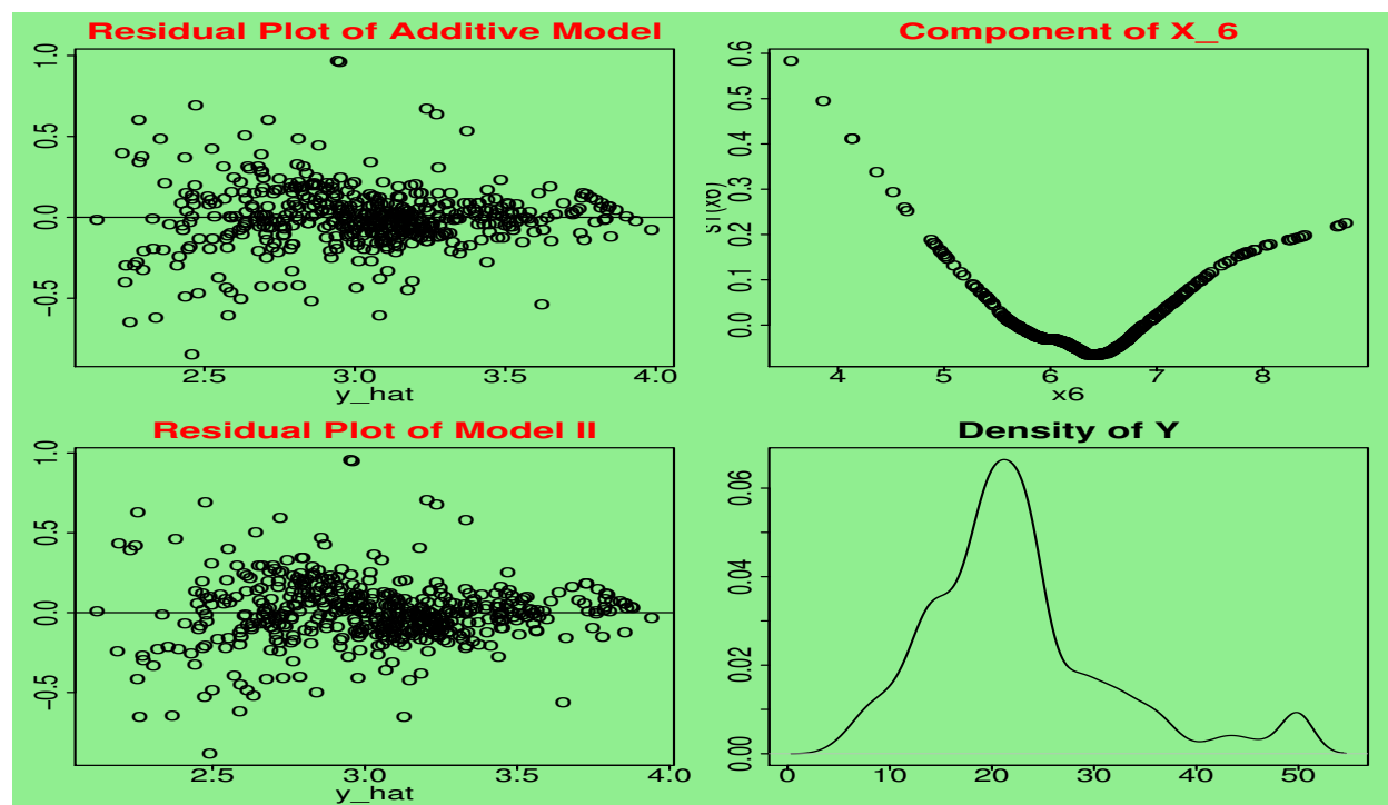
Figure 2.5: (a) Residual plot for model (2.67). (b) Plot of g_1(x_6) versus x_6 . (c) Residual plot for model (2.68). (d) Density estimate of Y .
